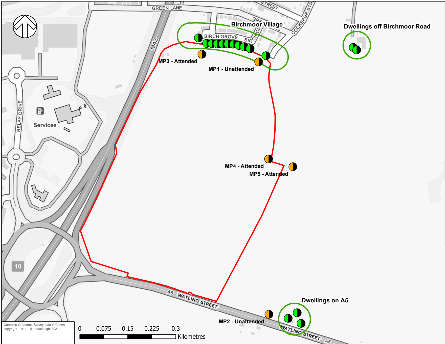
Figure 7.1 - Noise measurement locations and sensitive receptors
