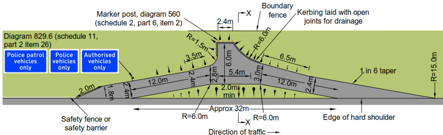
Figure 11.4.1a Observation platform type 1: drive-through platform
