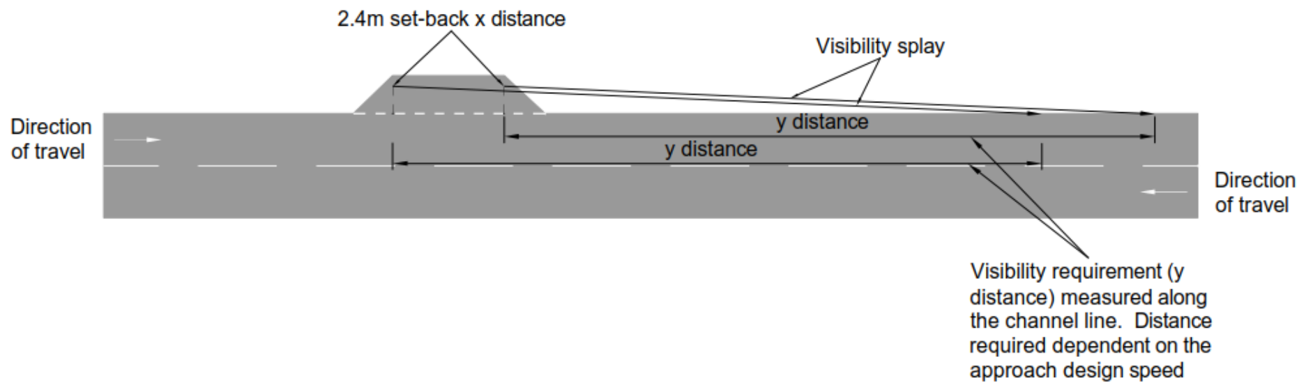
Figure 3.17Na Visibility requirements at the exit from a type B parking lay-by - opposite lane
